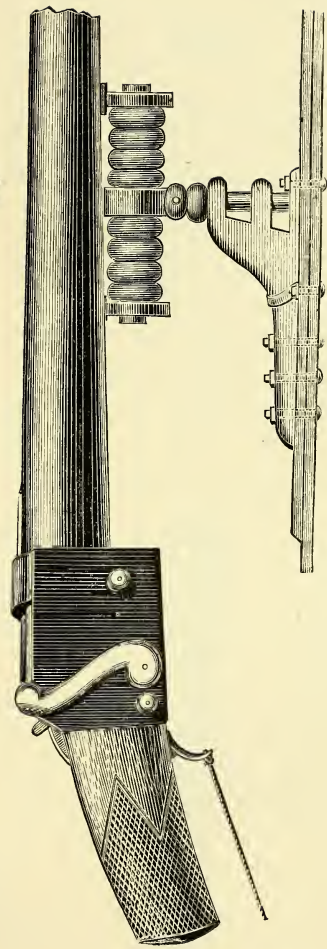
Greener-Field Punt Gun, with Indiarrubber Recoil-breeching.
